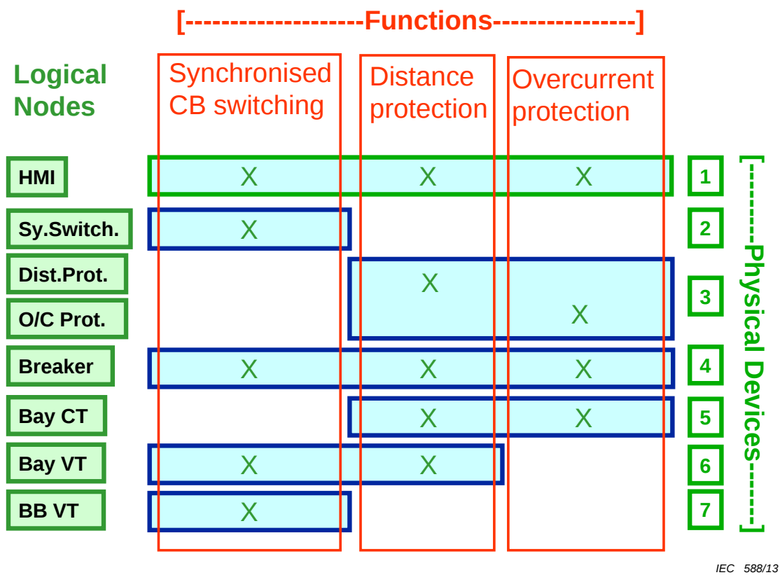
Figure 5 – Relationship between functions, logical nodes, and physical nodes (examples)
